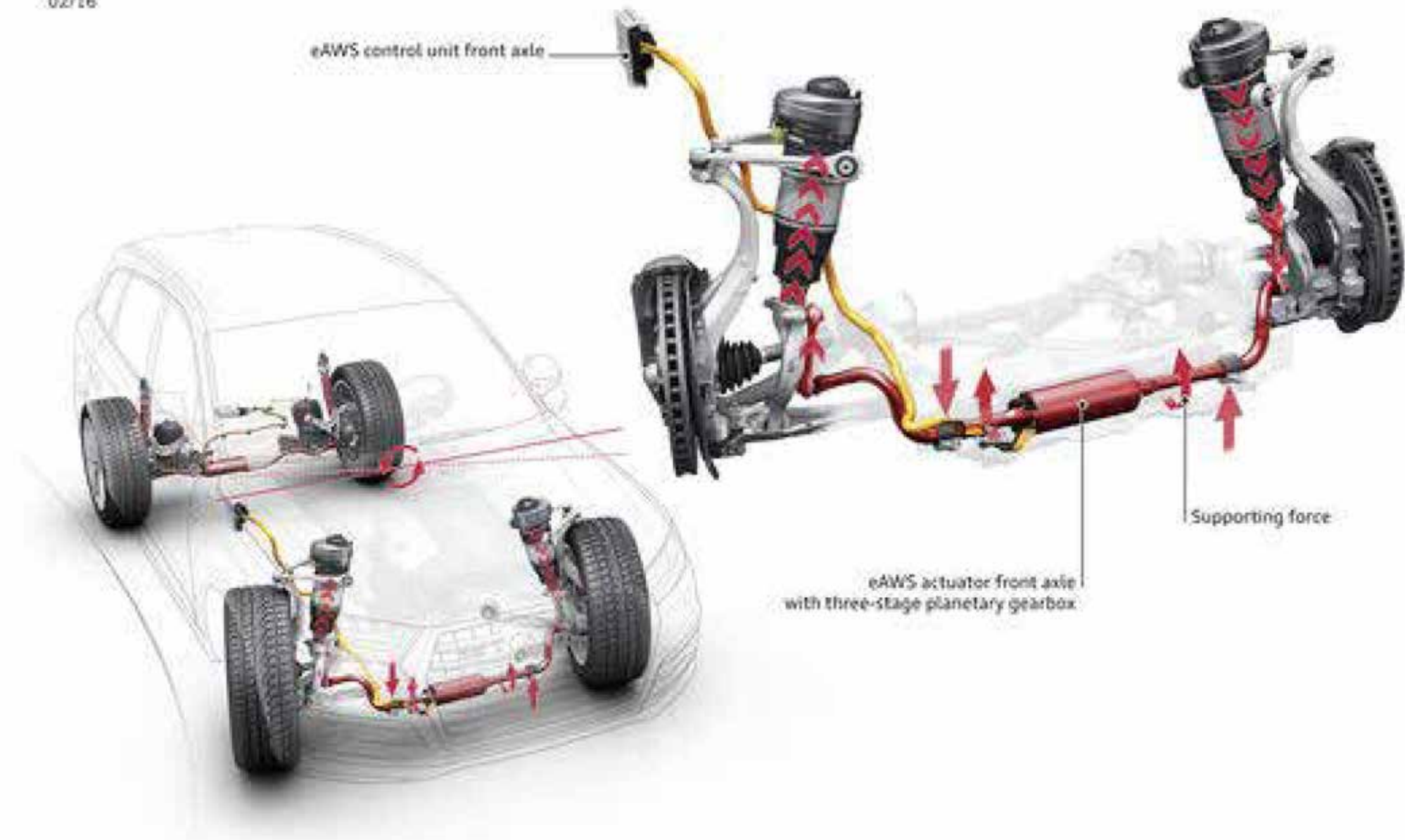
Audi SQ7 TDI electro-mechanical active roll stabilization (eAWS) 02/16
